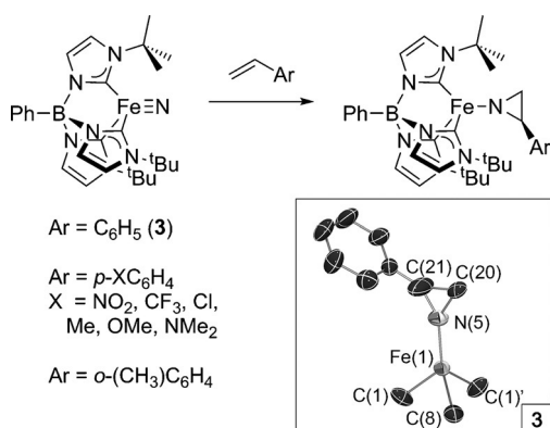
Scheme 1. Reaction of 1 with a range of styrenes, leading to formation of the corresponding aziridino complexes. Inset: X-ray crystal structure of 3 , where Ar = \text{C}_6\text{H}_5 . Thermal ellipsoids at 50%, hydrogen atoms and most of the tris(carbene)borate ligand omitted for clarity. Fe(1)–N(5) 1.935(4); Fe(1)–C(1) 2.092(4); Fe(1)–C(8) 2.109(6); N(5)–C(20) 1.417(11); N(5)–C(21) 1.317(14); C(20)–C(21) 1.476; C(1)–Fe(1)–C(8) 90.58(16); Fe(1)–N(5)–C(20) 142.0(5); Fe(1)–N(5)–C(21) 152.5(6); C(20)–N(5)–C(21) 65.3(6).
