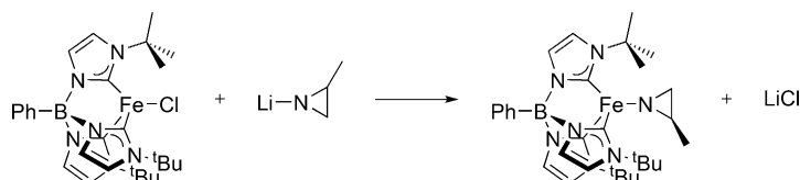
Scheme 4. Synthesis of [\text{PhB}(\text{tBuIm})_3\text{Fe-N}(\text{CH}_2\text{CHCH}_3)] ( 6 ).
