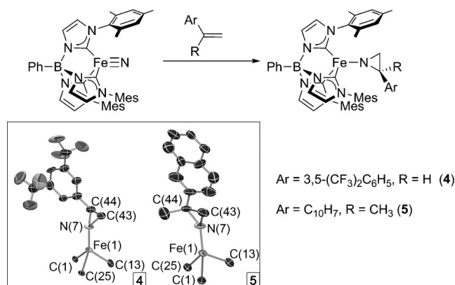
Scheme 2. Reaction of 2 with bulky styrenes to afford the corresponding aziridino complexes 4 and 5 . Inset: X-ray crystal structures of 4 (left) and 5 (right). Thermal ellipsoids at 50%, hydrogen atoms and most of the tris(carbene)borate ligand omitted for clarity.
