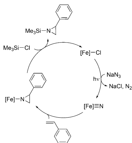
Scheme 5. Synthetic cycle for styrene aziridination by an iron(IV) nitride complex.
