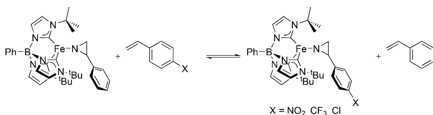
Scheme 3. Aziridine cross-metathesis.
