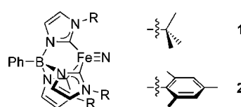
Figure 1. The iron(IV) nitrides [\text{PhB}(\text{RIm})_3\text{Fe}\equiv\text{N}] ( \text{R} = \text{tBu} 1 , \text{Mes} 2 ).
